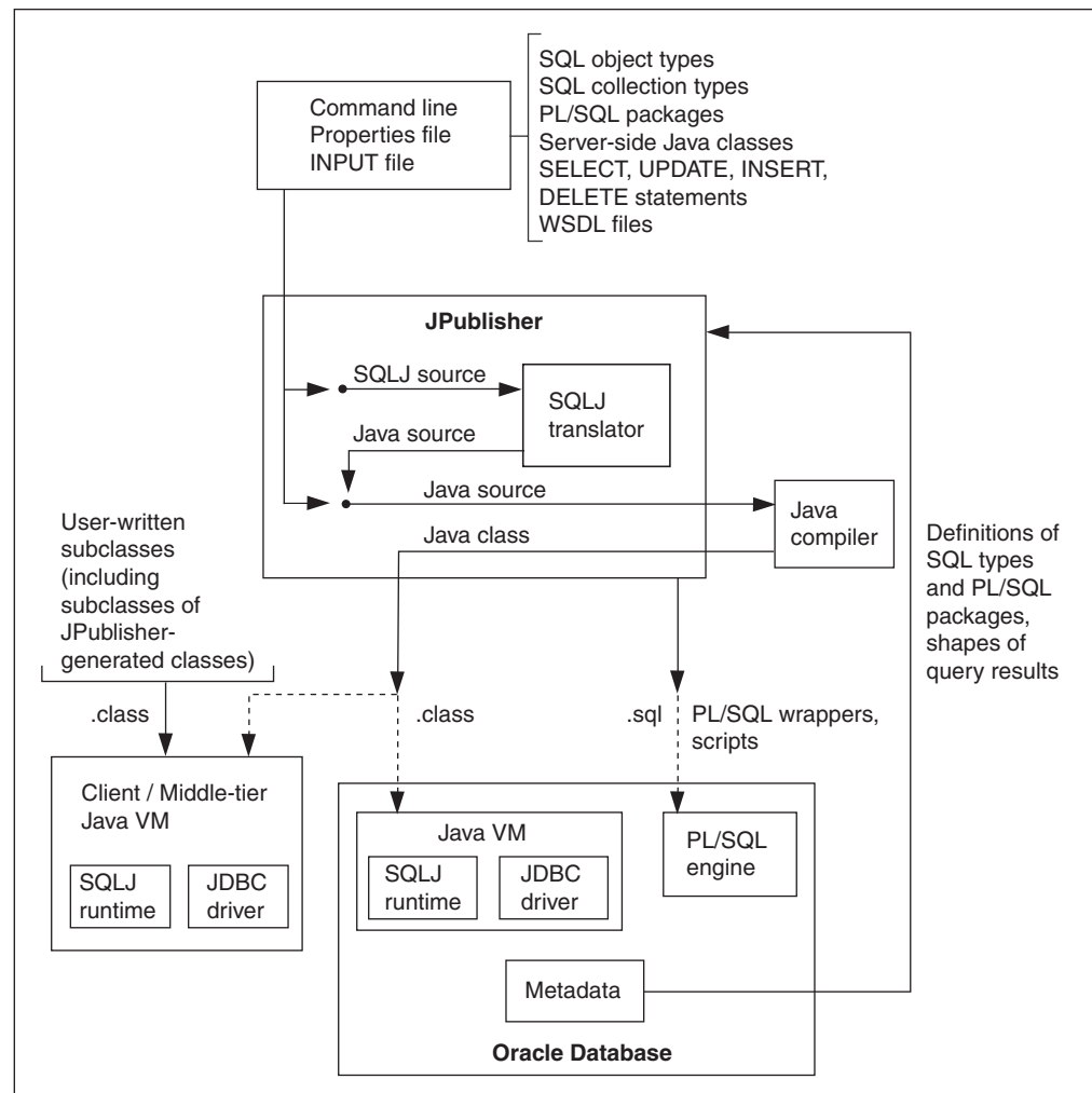
Figure 1–8 Translating and Using JPublisher-Generated Code
