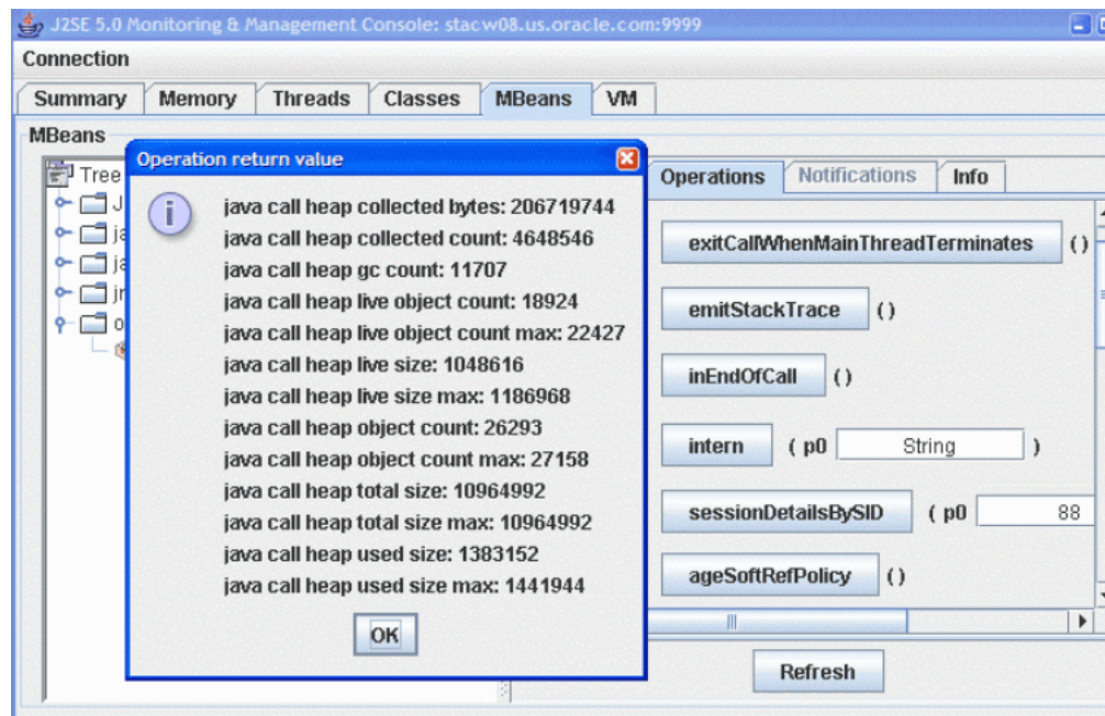
Figure 2–18 Operation sessionDetailsBySID
