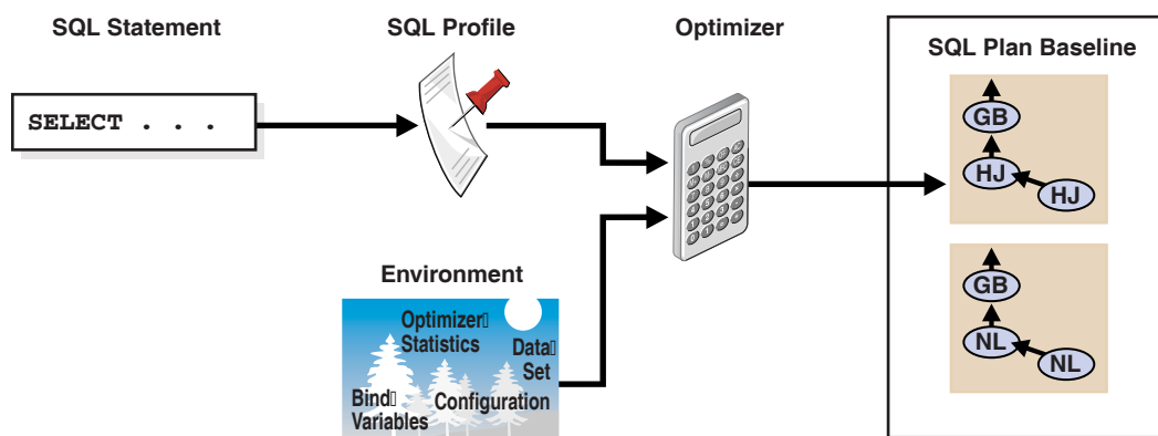
Figure 17–4 SQL Profile
