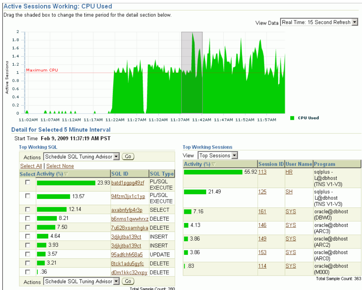
Figure 9–2 Viewing SQL Statements by Wait Class
