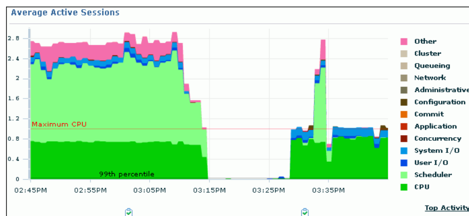
Figure 4–2 Monitoring User Activity
