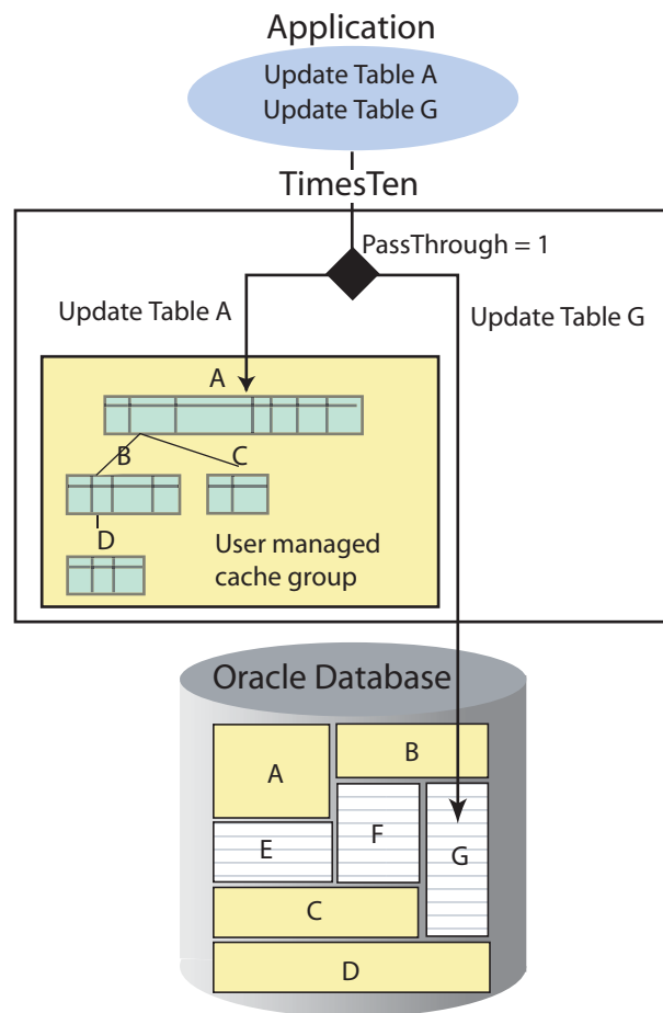
Figure 5-1 Behavior of the PassThrough=1 setting
